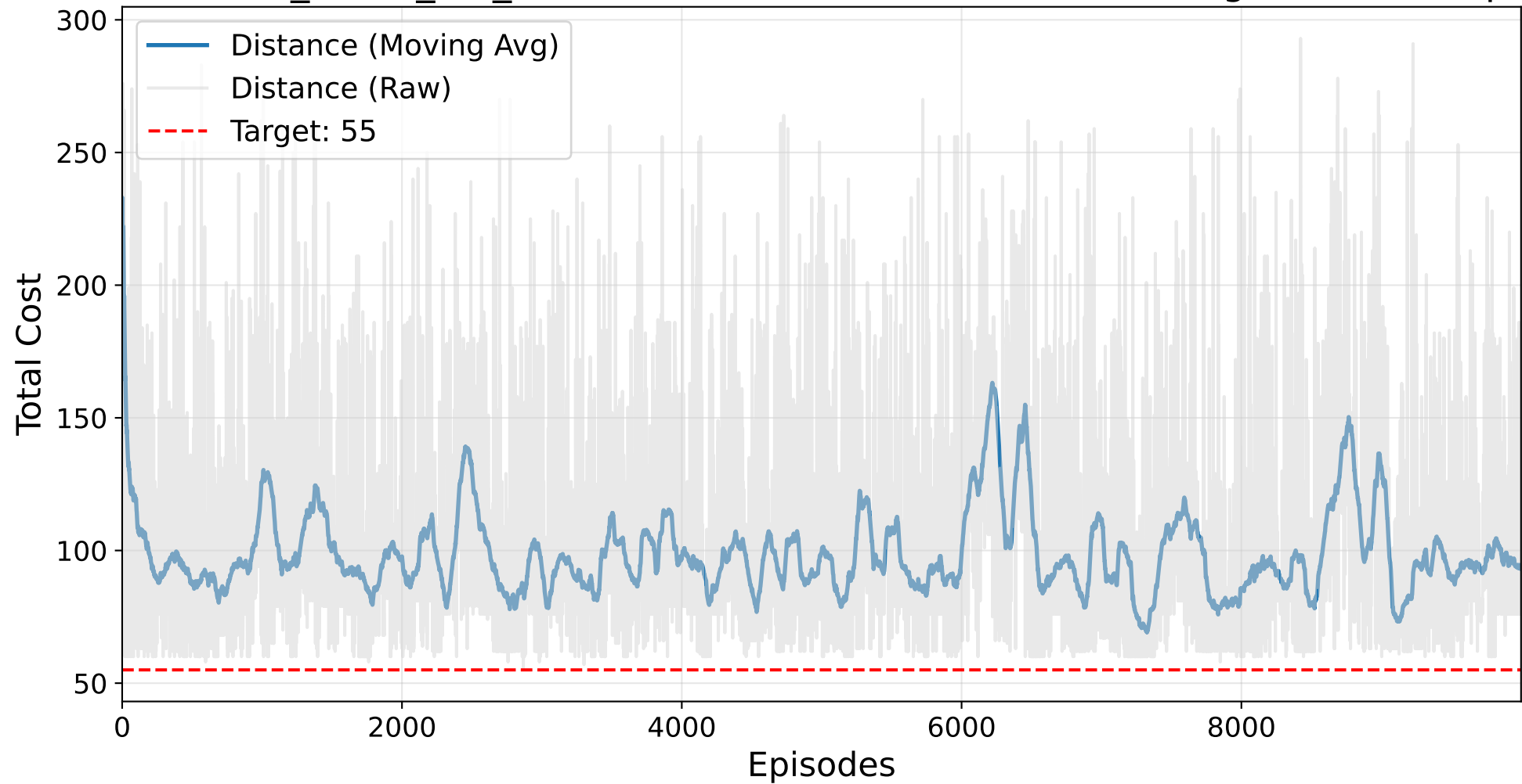
Final NO_MASK_NO_BAYESIAN Masked AutoRL-SOP Training - br17.10.sop
